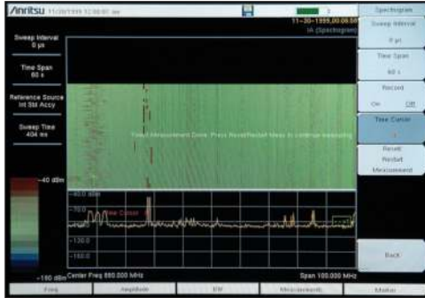
Spectrogram Display
