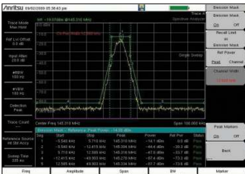
Emission Mask Measurements
